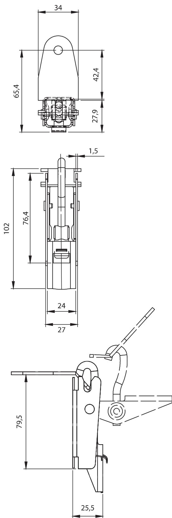
7402 - Latch
