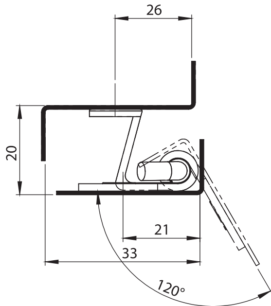
3045 - 120° Consealed Hinge
