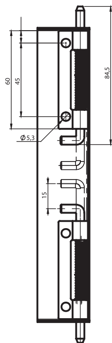
3025 - 120° Consealed Hinge
