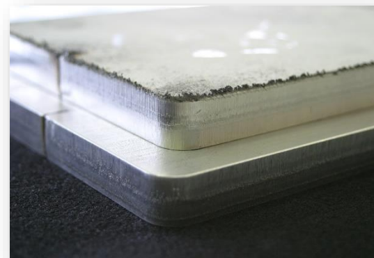
Piese taiate la Laser
